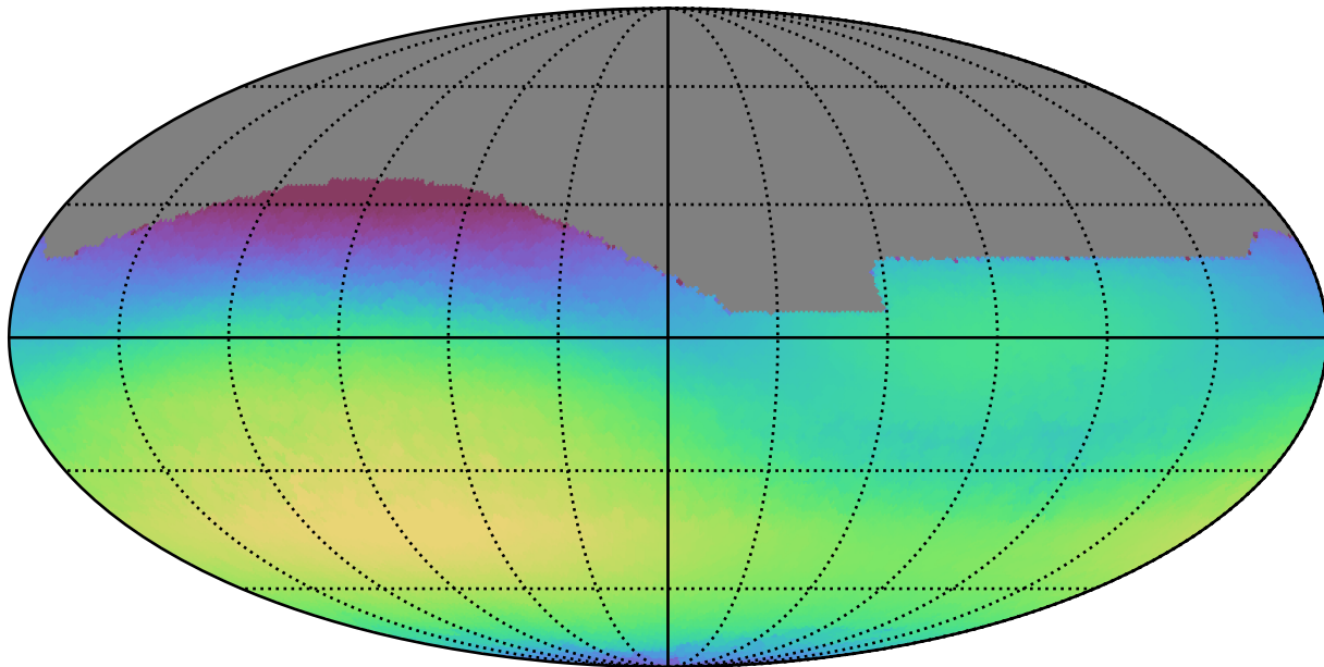
too_elab_r32_d2_giz_v3.4_10yrs All sky r band: Max skyBrightness
