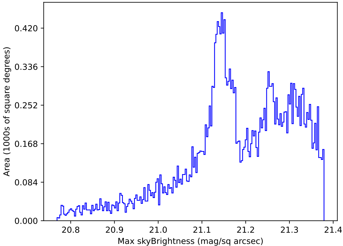
too_elab_r32_d2_giz_v3.4_10yrs All sky r band: Max skyBrightness
