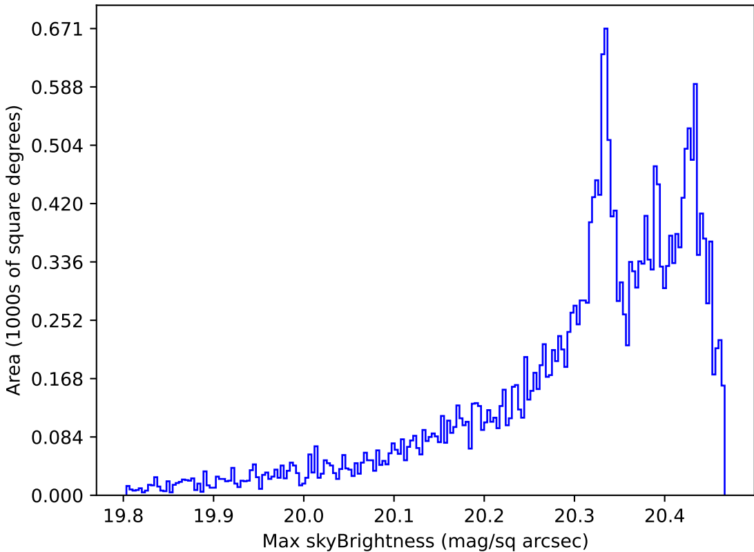
too_elab_r32_d2_giz_v3.4_10yrs All sky i band: Max skyBrightness
