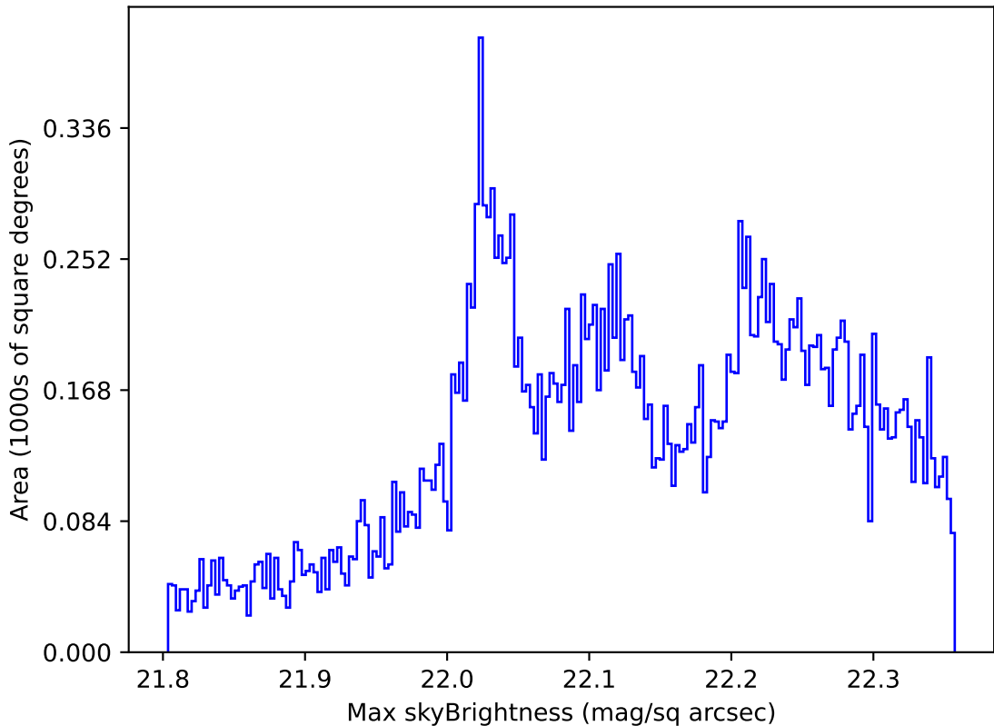
too_elab_r32_d2_giz_v3.4_10yrs All sky g band: Max skyBrightness
