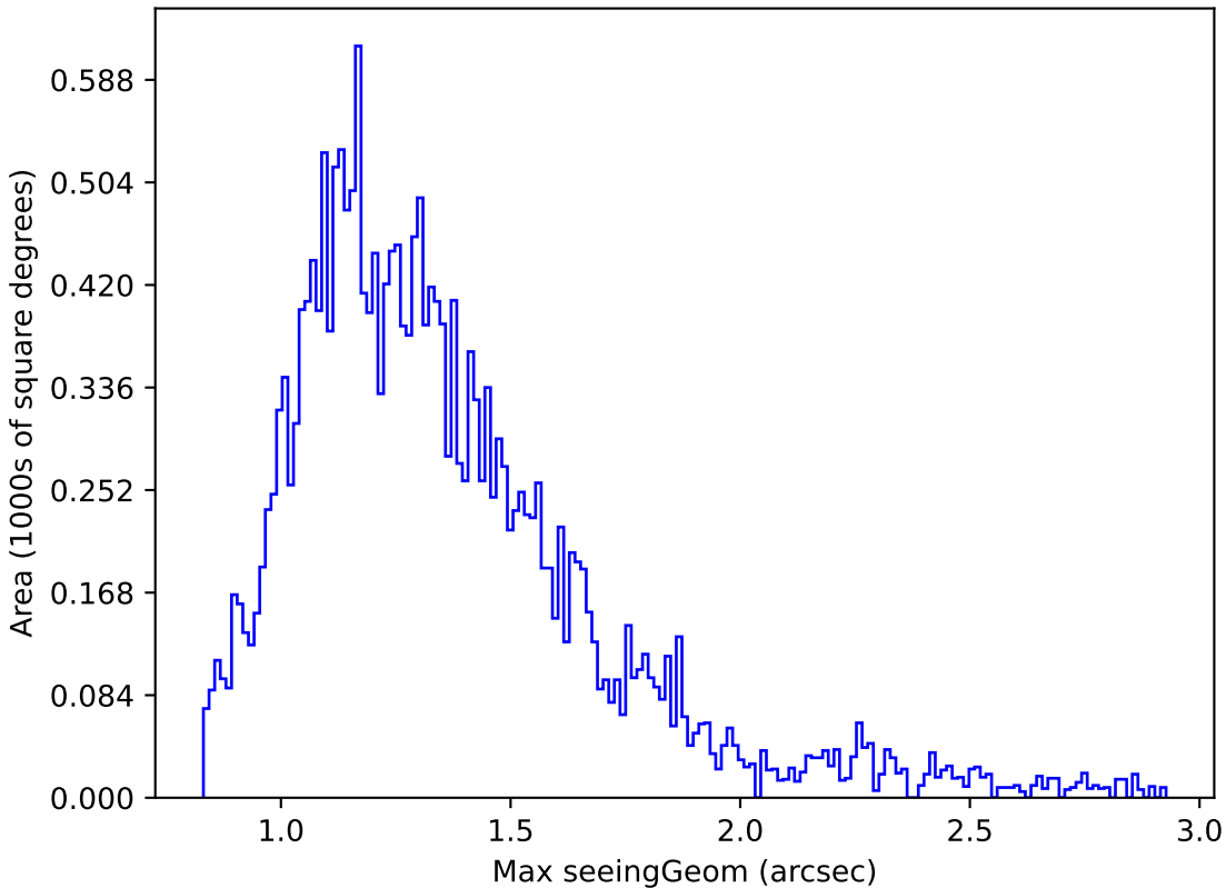
too_elab_r32_d2_giz_v3.4_10yrs Yr 1 u band: Max seeingGeom
