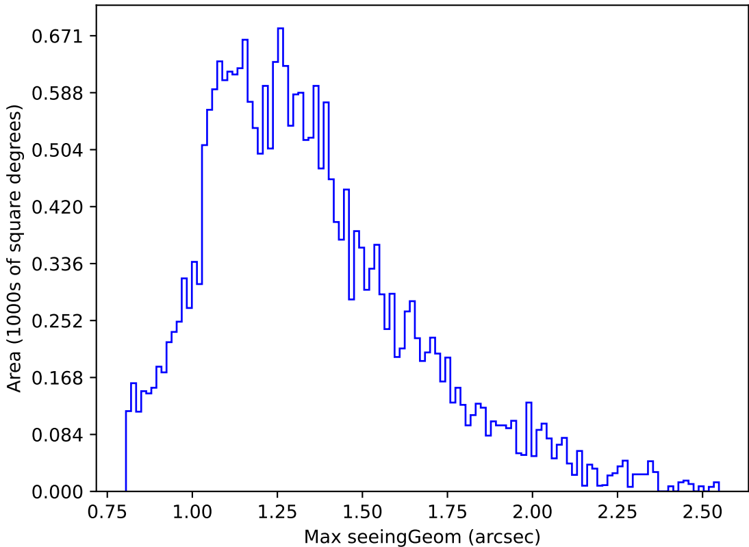
too_elab_r32_d2_giz_v3.4_10yrs Yr 1 g band: Max seeingGeom
