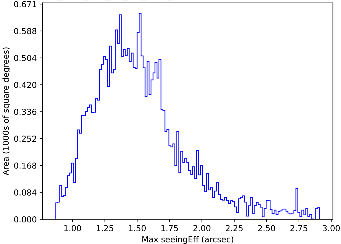
too_elab_r32_d2_giz_v3.4_10yrs Yr 1 z band: Max seeingEff
