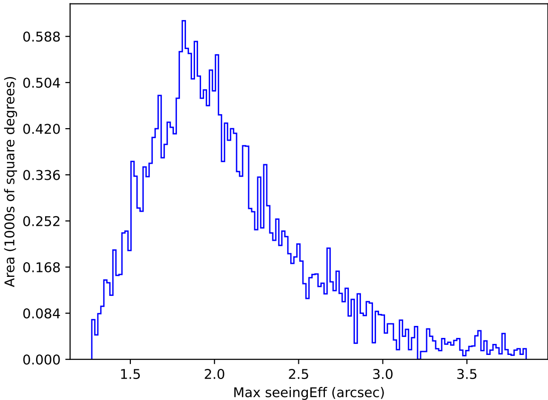
too_elab_r32_d2_giz_v3.4_10yrs Yr 1 all bands: Max seeingEff
