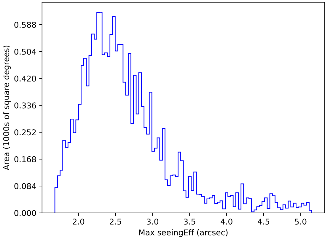
too_elab_r32_d2_giz_v3.4_10yrs WFD z band: Max seeingEff
