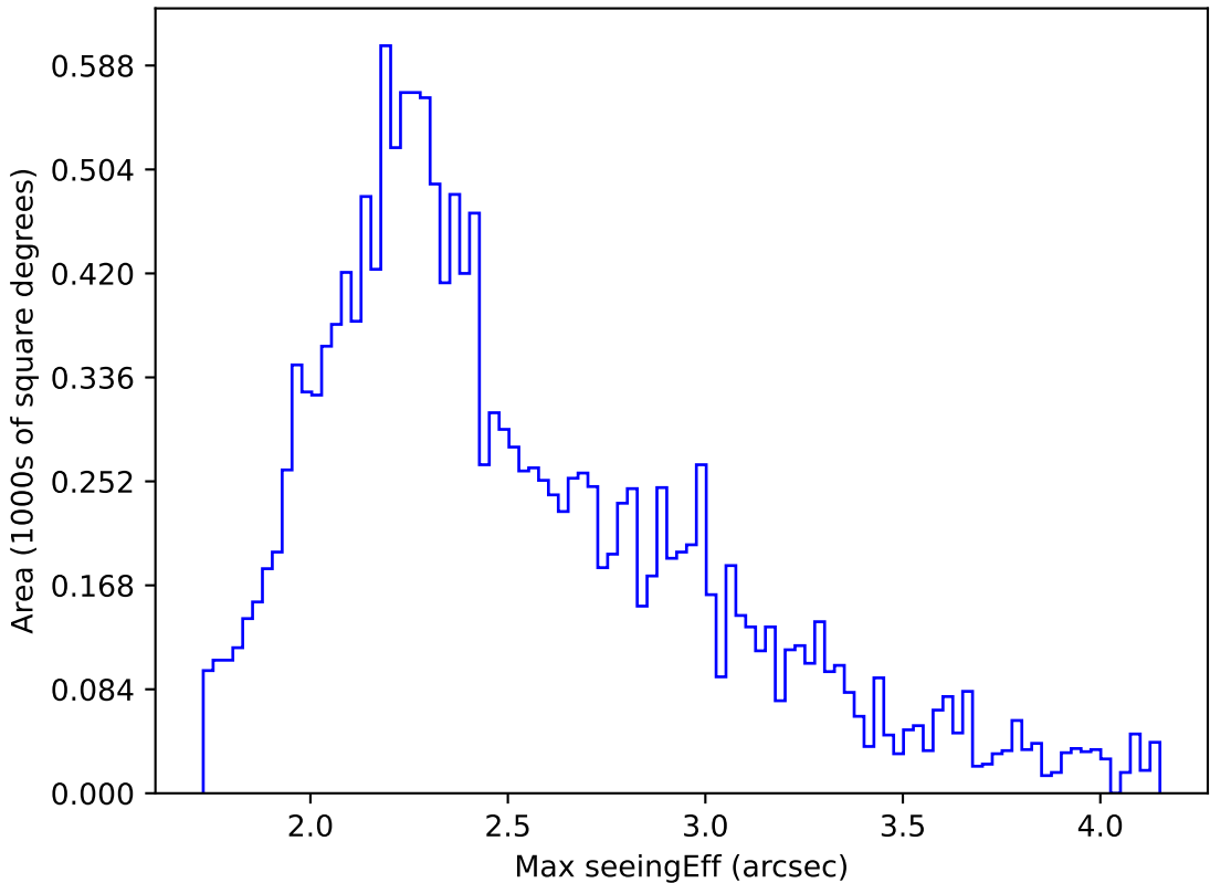
too_elab_r32_d2_giz_v3.4_10yrs WFD u band: Max seeingEff
