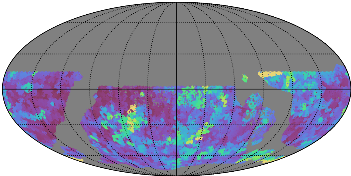
too_elab_r32_d2_giz_v3.4_10yrs WFD g band: Max seeingEff
