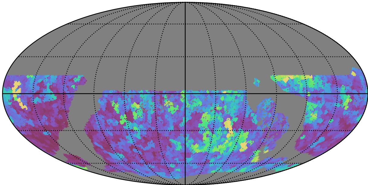
too_elab_r32_d2_giz_v3.4_10yrs WFD all bands: Max seeingEff
