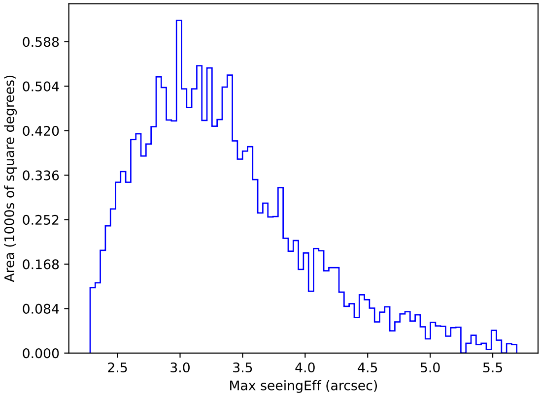
too_elab_r32_d2_giz_v3.4_10yrs WFD all bands: Max seeingEff
