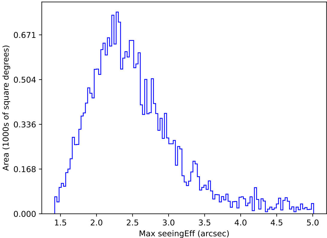
too_elab_r32_d2_giz_v3.4_10yrs All sky z band: Max seeingEff
