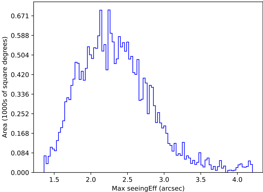
too_elab_r32_d2_giz_v3.4_10yrs All sky y band: Max seeingEff
