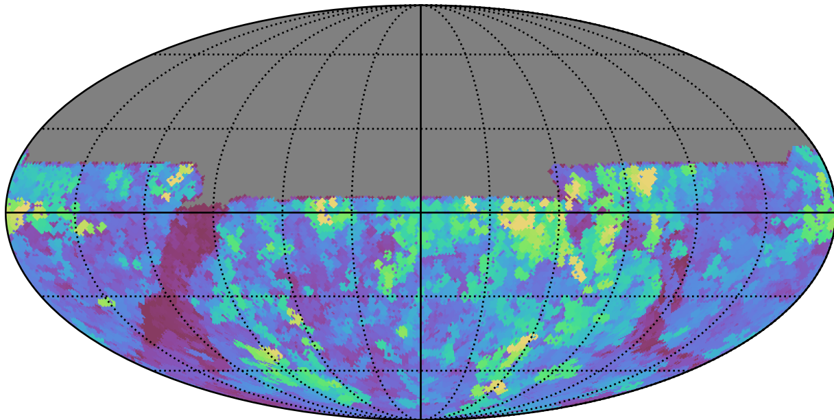
too_elab_r32_d2_giz_v3.4_10yrs All sky u band: Max seeingEff
