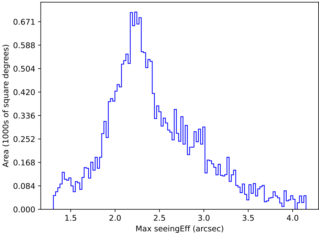
too_elab_r32_d2_giz_v3.4_10yrs All sky u band: Max seeingEff
