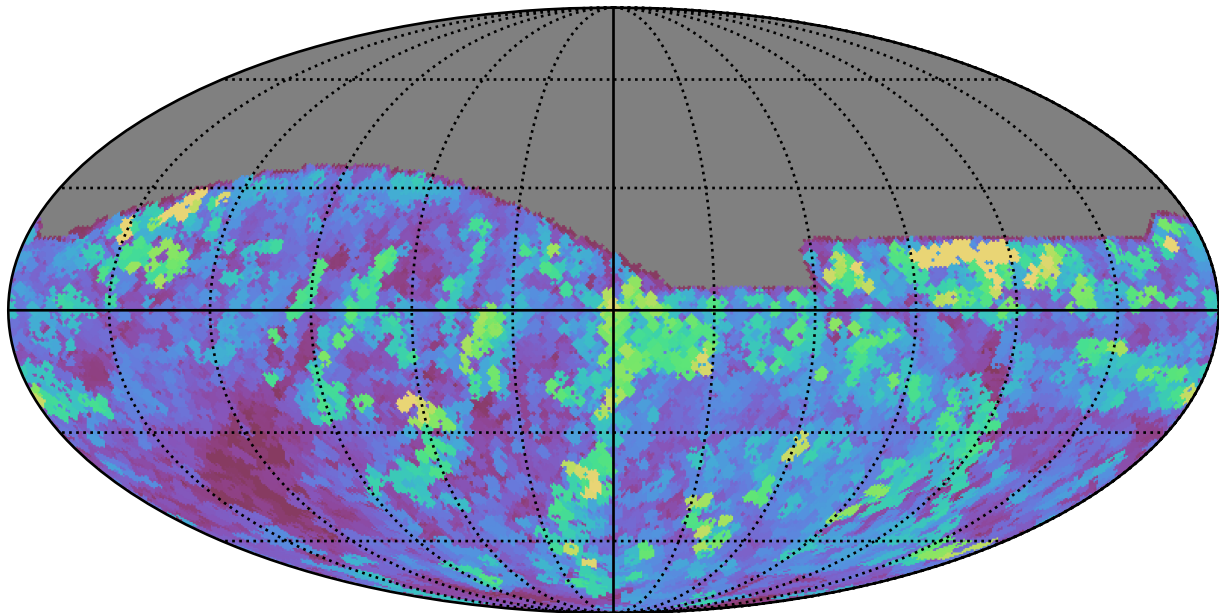
too_elab_r32_d2_giz_v3.4_10yrs All sky r band: Max seeingEff
