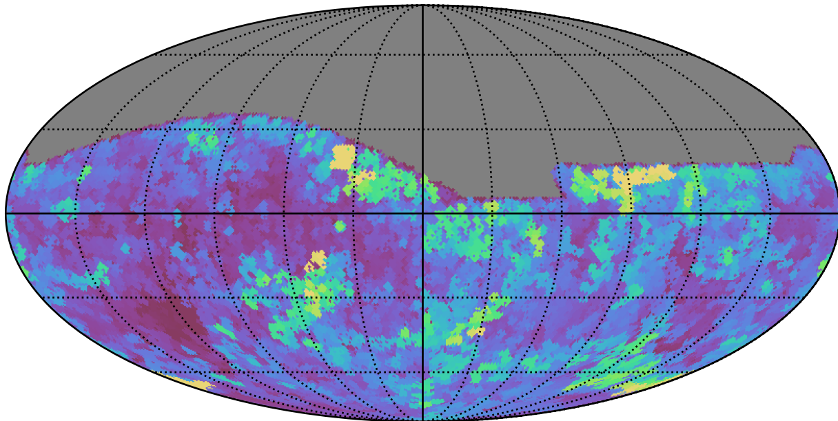
too_elab_r32_d2_giz_v3.4_10yrs All sky g band: Max seeingEff
