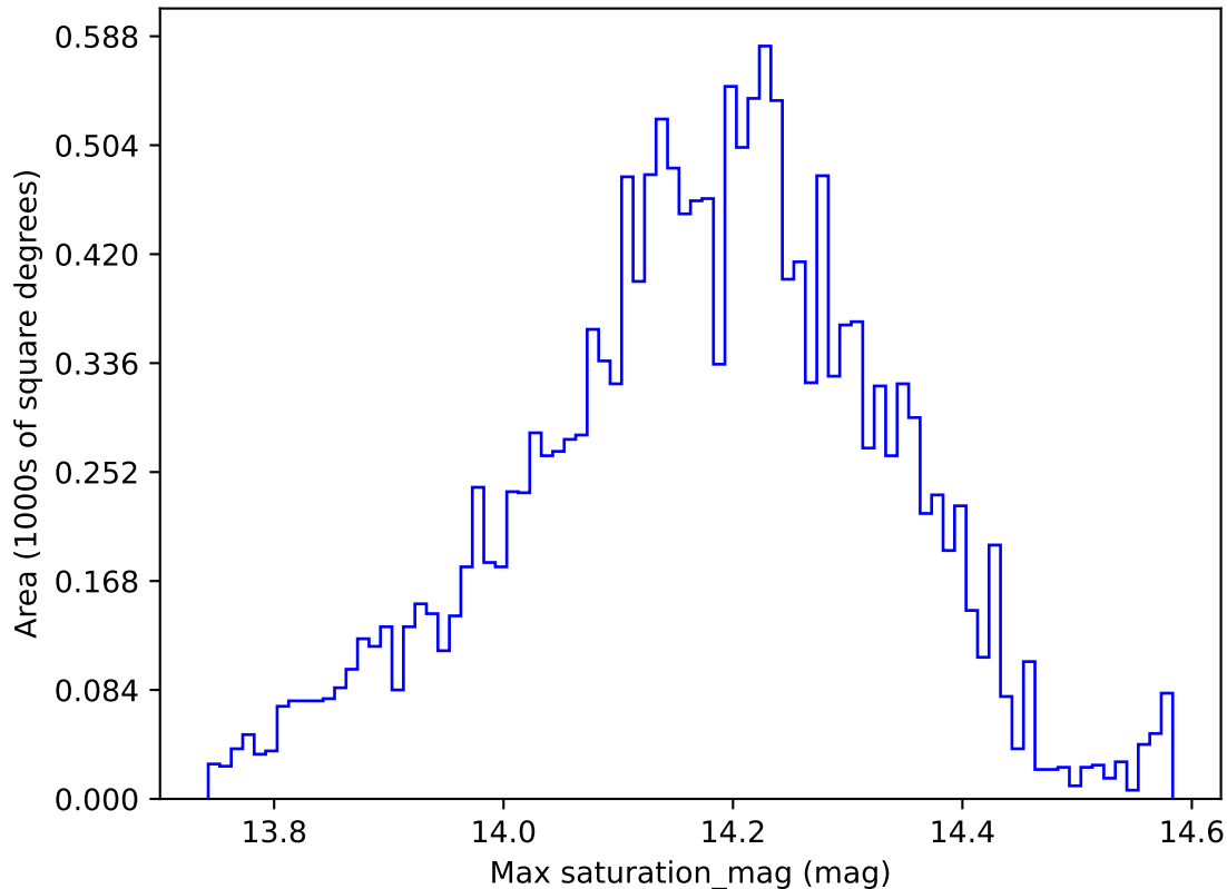
too_elab_r32_d2_giz_v3.4_10yrs WFD y band: Max saturation_mag
