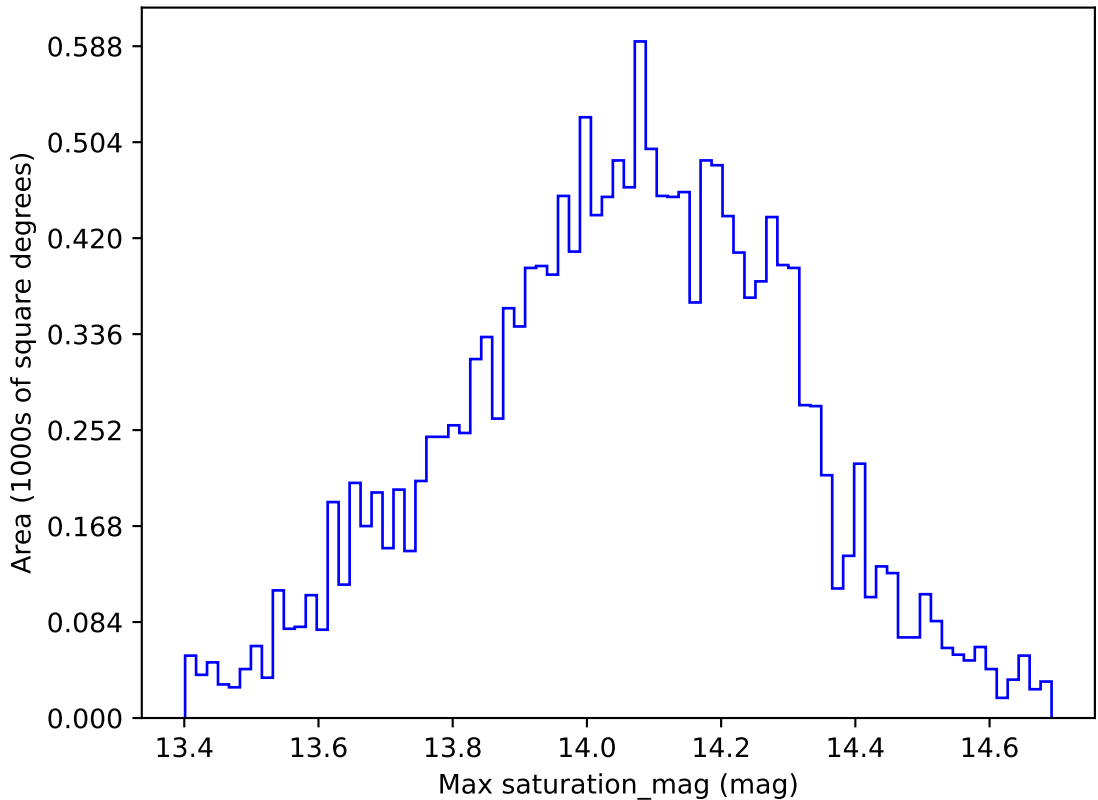
too_elab_r32_d2_giz_v3.4_10yrs WFD u band: Max saturation_mag
