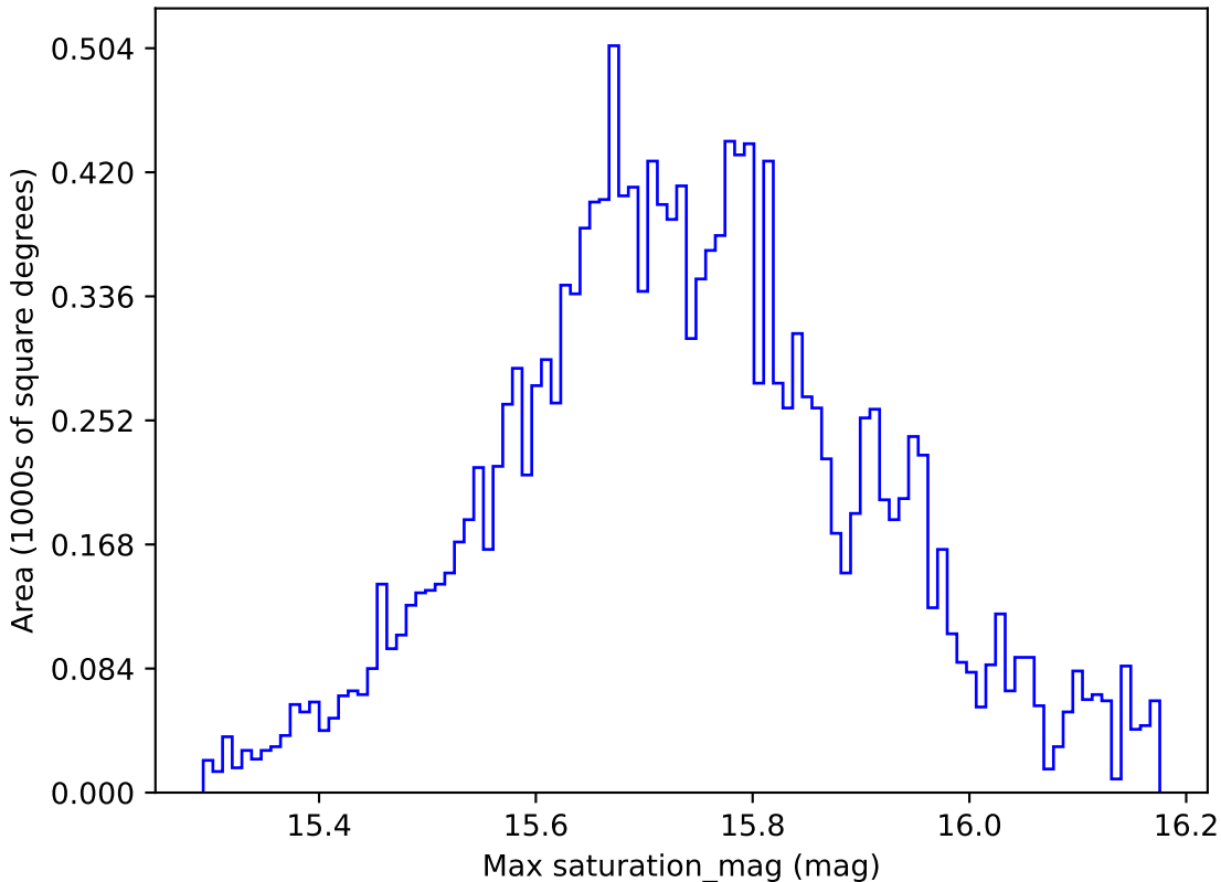
too_elab_r32_d2_giz_v3.4_10yrs WFD g band: Max saturation_mag
