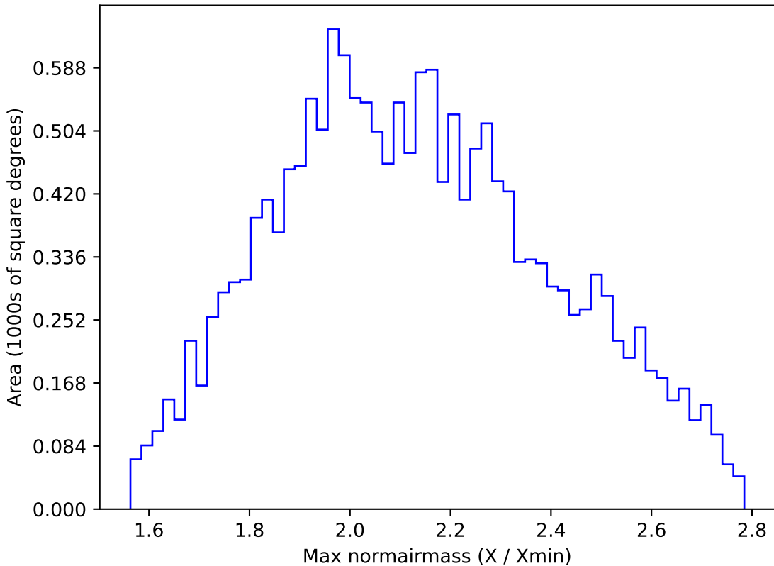
too_elab_r32_d2_giz_v3.4_10yrs WFD y band: Max normairmass
