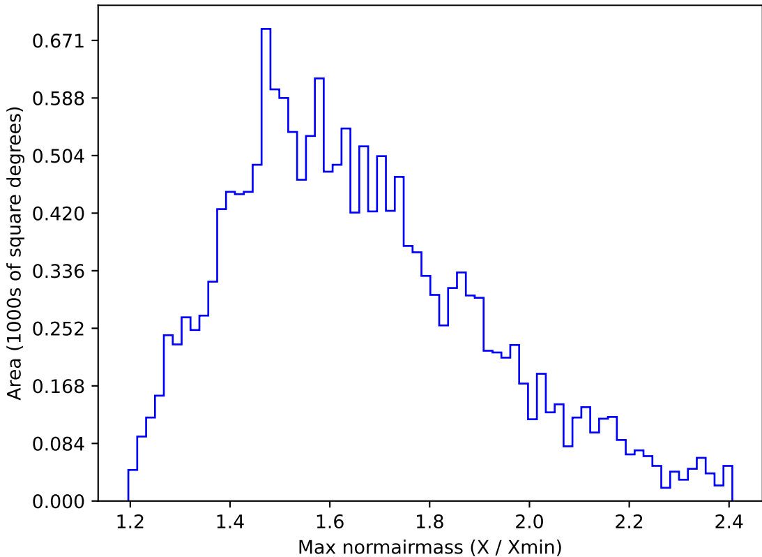
too_elab_r32_d2_giz_v3.4_10yrs WFD u band: Max normairmass
