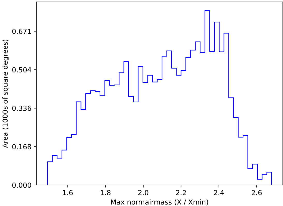
too_elab_r32_d2_giz_v3.4_10yrs WFD r band: Max normairmass
