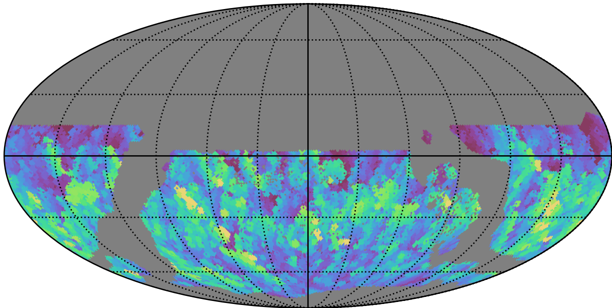
too_elab_r32_d2_giz_v3.4_10yrs WFD g band: Max normairmass
