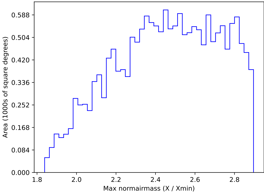
too_elab_r32_d2_giz_v3.4_10yrs WFD all bands: Max normairmass
