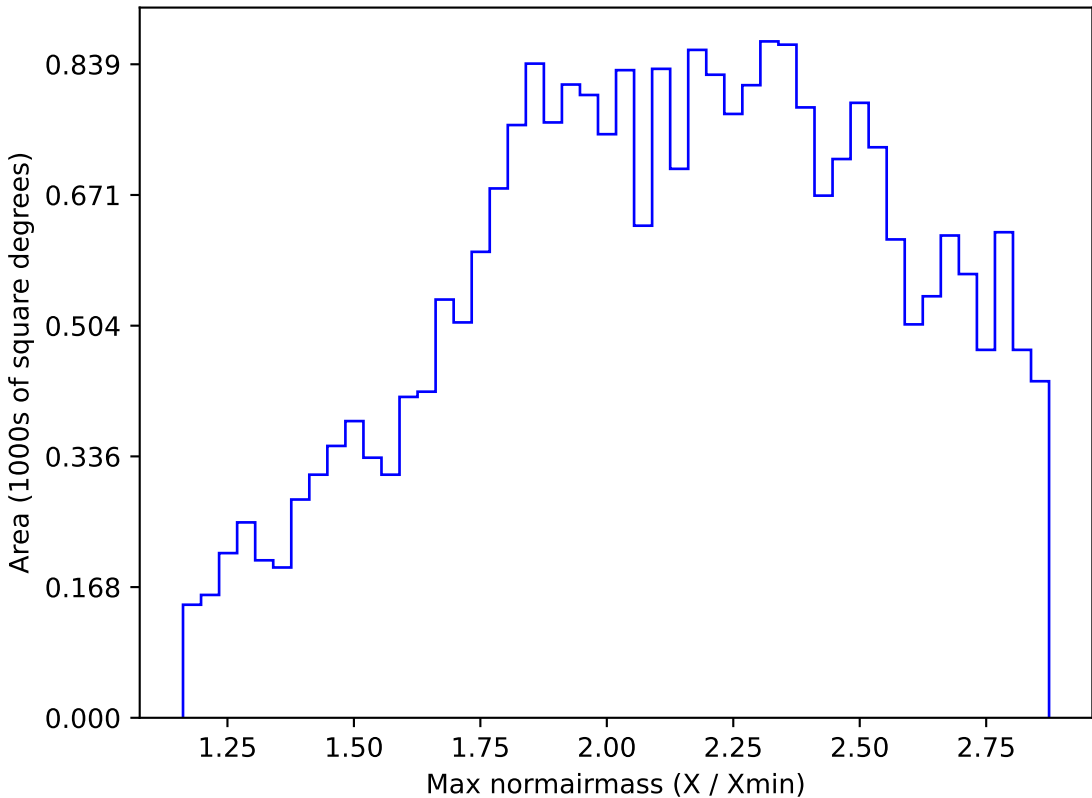
too_elab_r32_d2_giz_v3.4_10yrs All sky z band: Max normairmass
