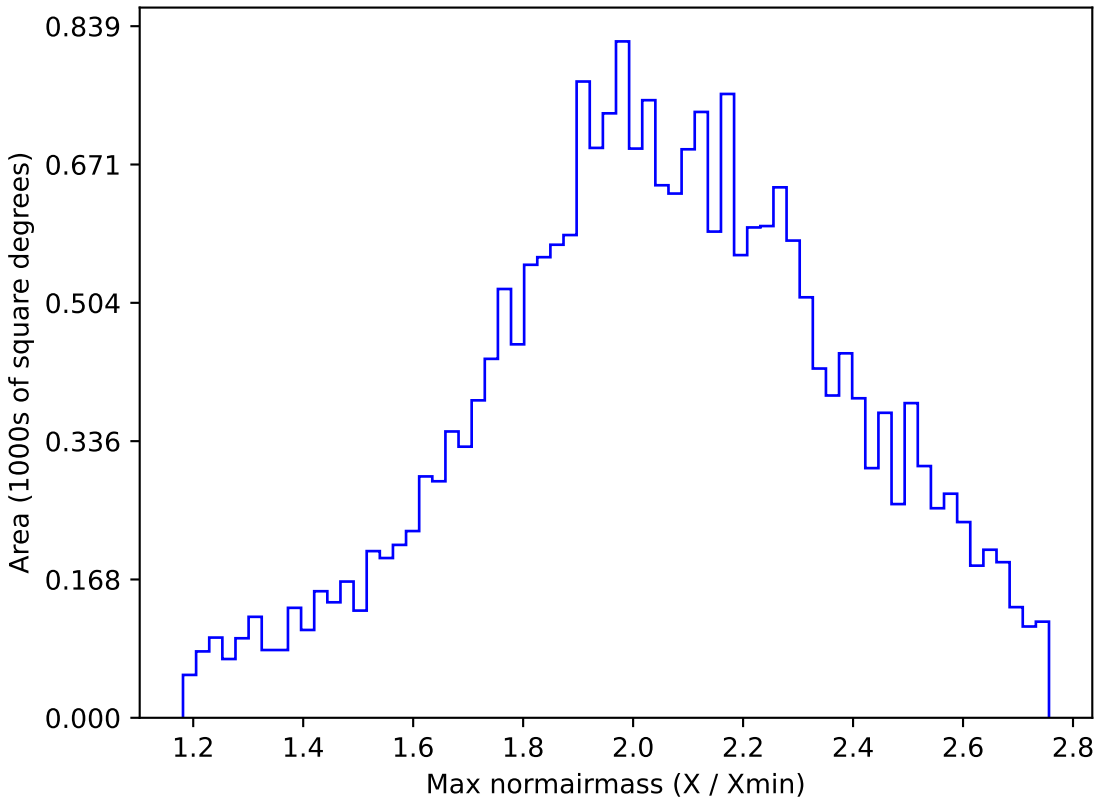
too_elab_r32_d2_giz_v3.4_10yrs All sky y band: Max normairmass
