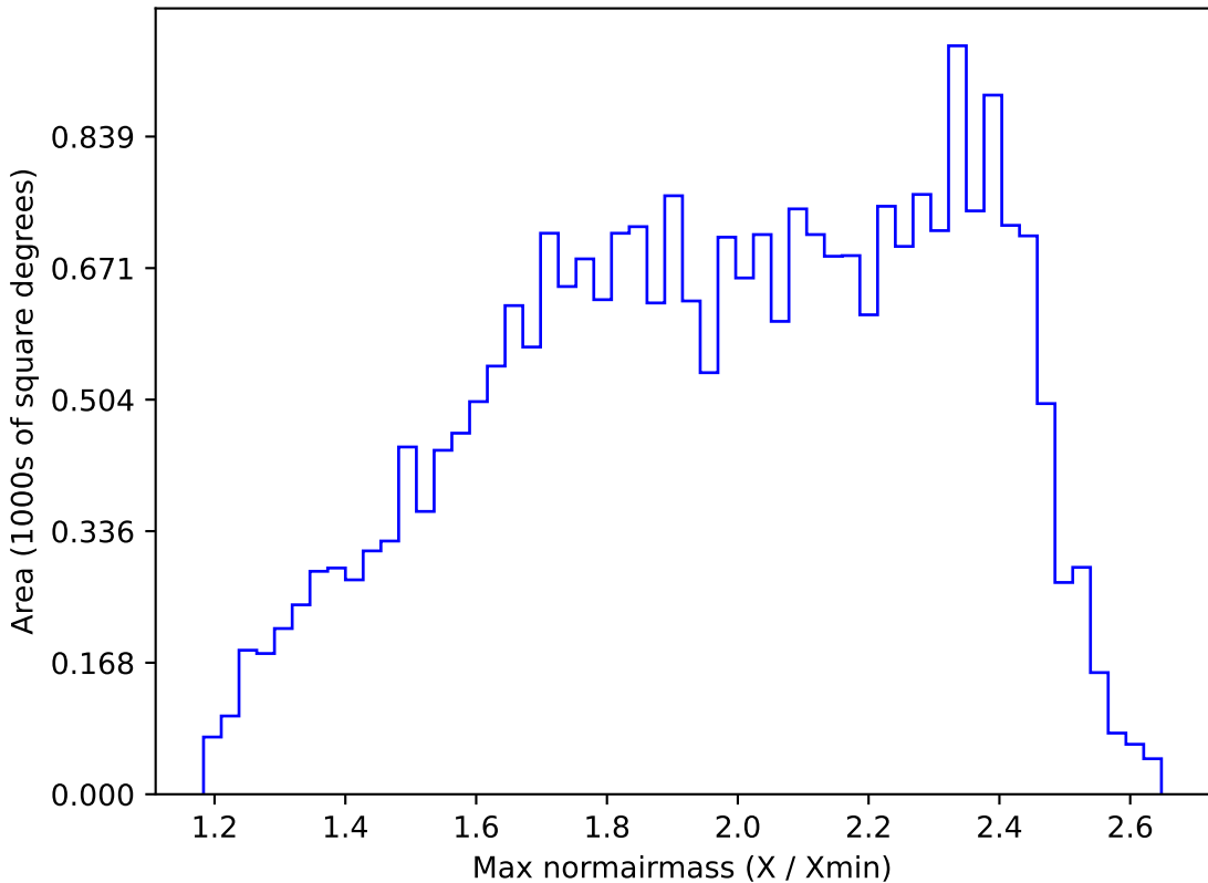
too_elab_r32_d2_giz_v3.4_10yrs All sky r band: Max normairmass
