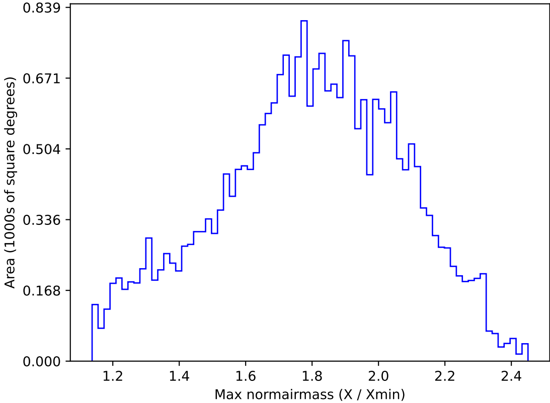
too_elab_r32_d2_giz_v3.4_10yrs All sky g band: Max normairmass
