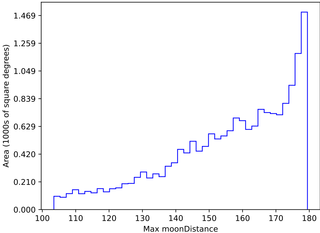
too_elab_r32_d2_giz_v3.4_10yrs WFD r band: Max moonDistance
