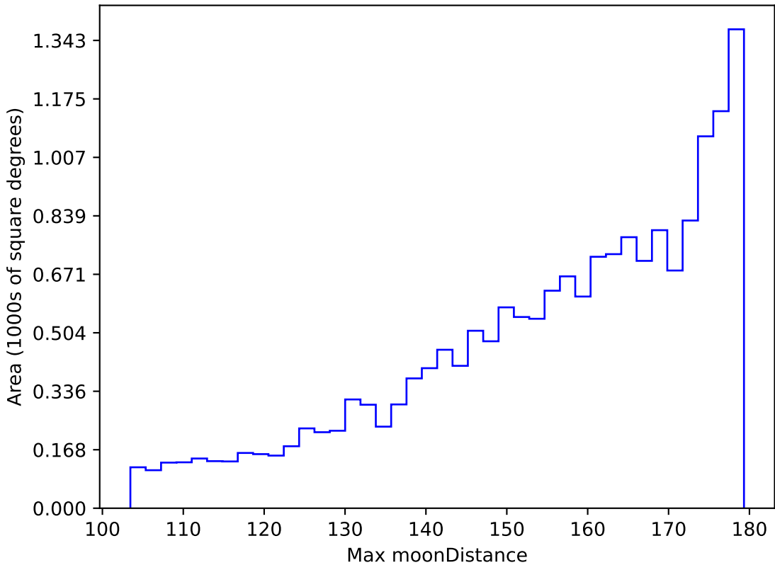
too_elab_r32_d2_giz_v3.4_10yrs WFD i band: Max moonDistance
