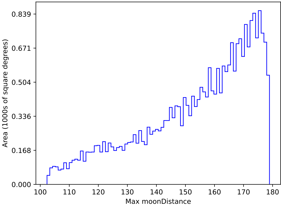
too_elab_r32_d2_giz_v3.4_10yrs All sky z band: Max moonDistance
