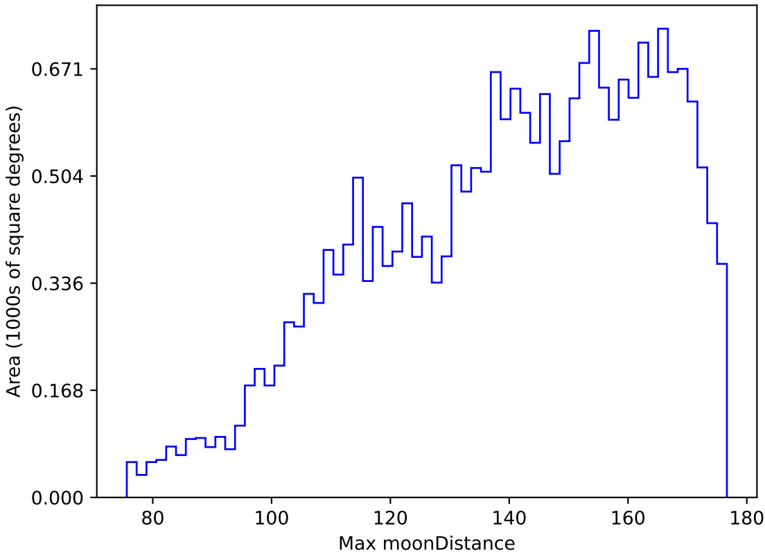
too_elab_r32_d2_giz_v3.4_10yrs All sky y band: Max moonDistance
