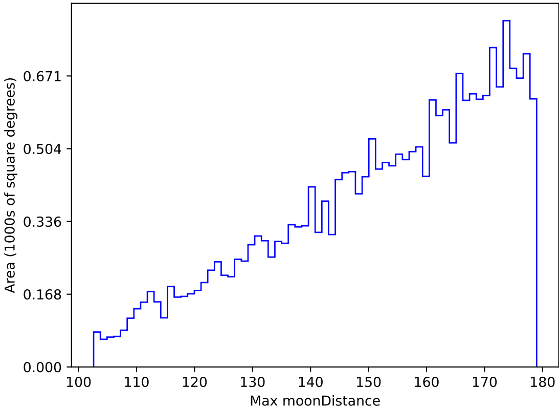
too_elab_r32_d2_giz_v3.4_10yrs All sky u band: Max moonDistance
