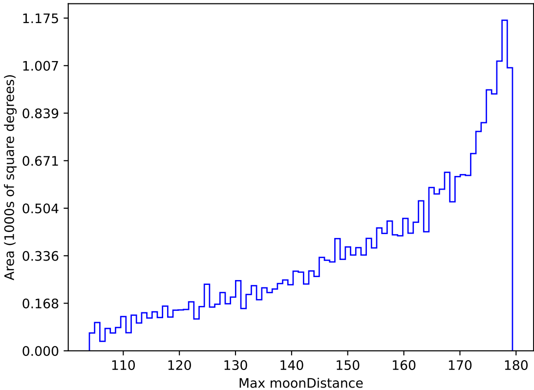
too_elab_r32_d2_giz_v3.4_10yrs All sky r band: Max moonDistance
