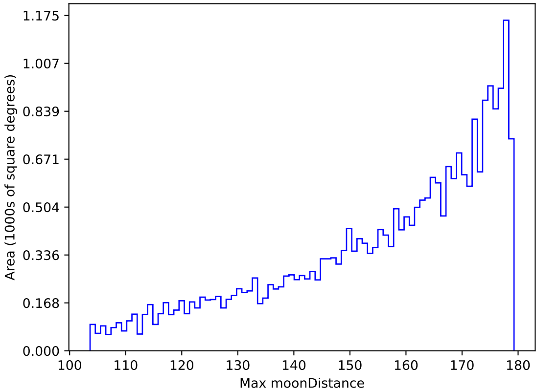
too_elab_r32_d2_giz_v3.4_10yrs All sky i band: Max moonDistance
