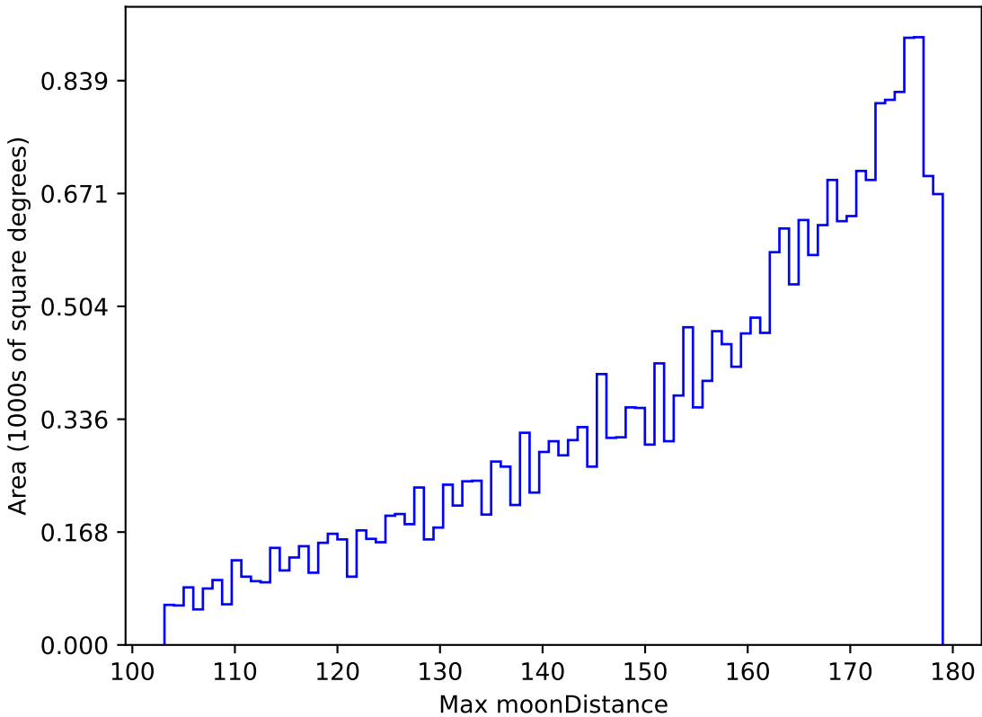
too_elab_r32_d2_giz_v3.4_10yrs All sky g band: Max moonDistance
