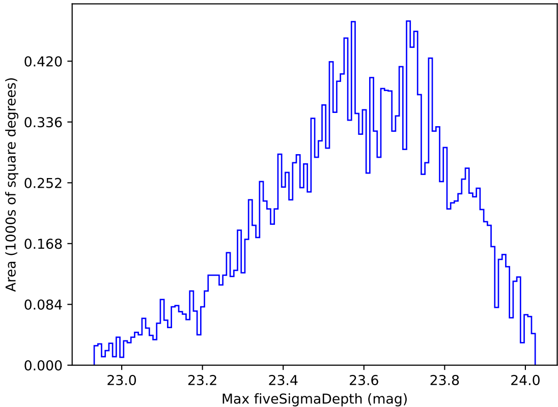
too_elab_r32_d2_giz_v3.4_10yrs Yr 1 u band: Max fiveSigmaDepth
