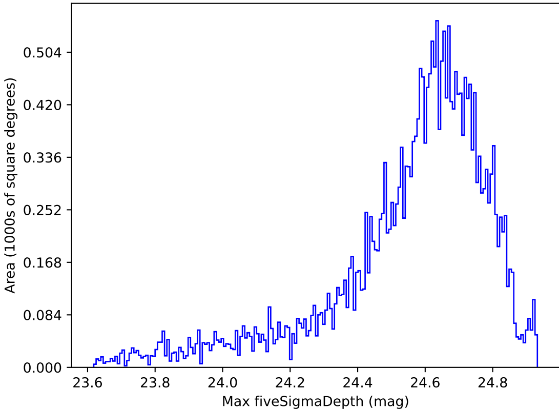
too_elab_r32_d2_giz_v3.4_10yrs Yr 1 r band: Max fiveSigmaDepth
