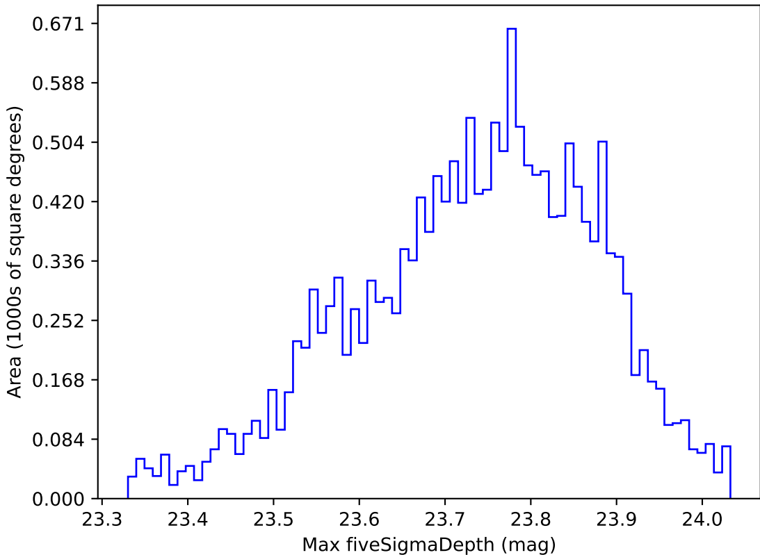
too_elab_r32_d2_giz_v3.4_10yrs WFD u band: Max fiveSigmaDepth
