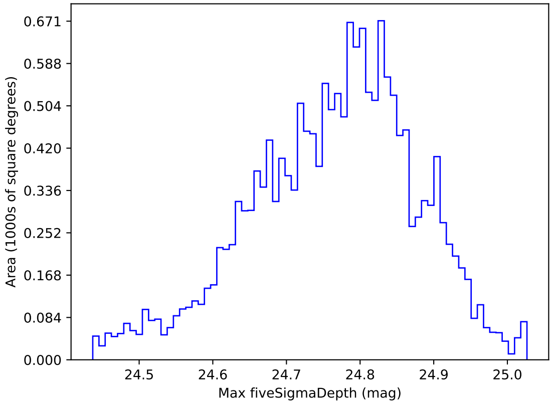
too_elab_r32_d2_giz_v3.4_10yrs WFD r band: Max fiveSigmaDepth
