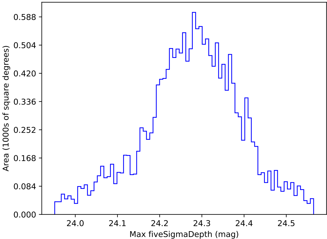
too_elab_r32_d2_giz_v3.4_10yrs WFD i band: Max fiveSigmaDepth
