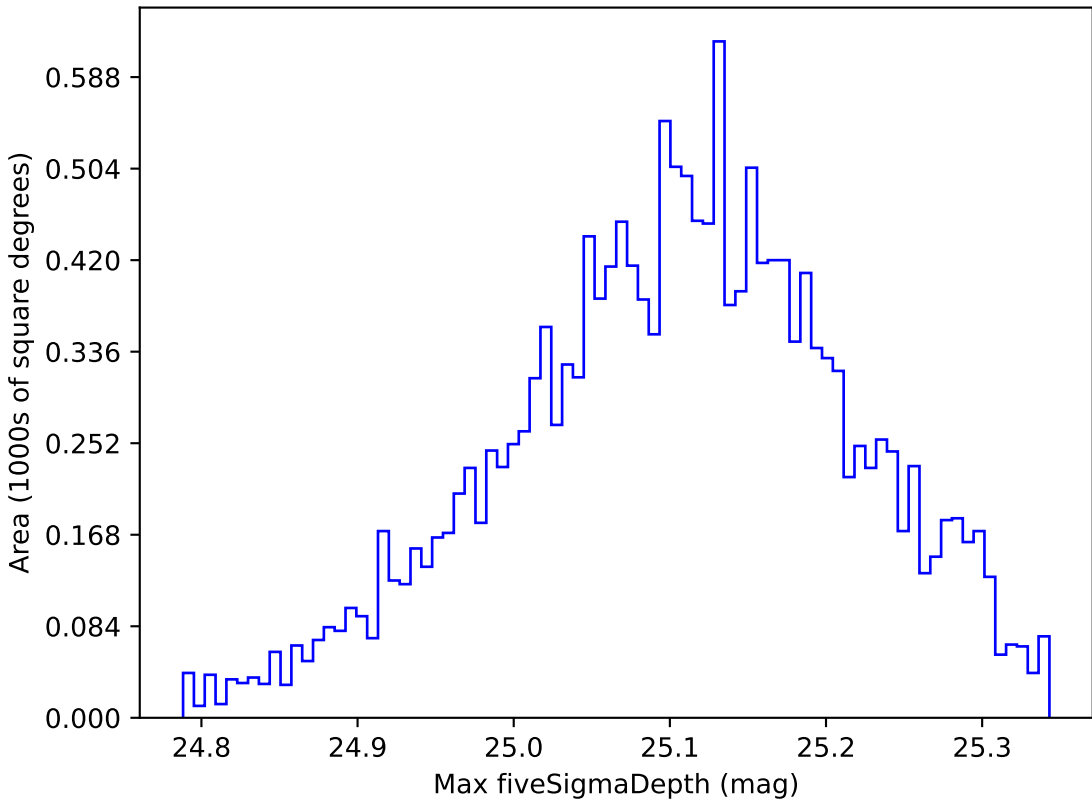
too_elab_r32_d2_giz_v3.4_10yrs WFD g band: Max fiveSigmaDepth
