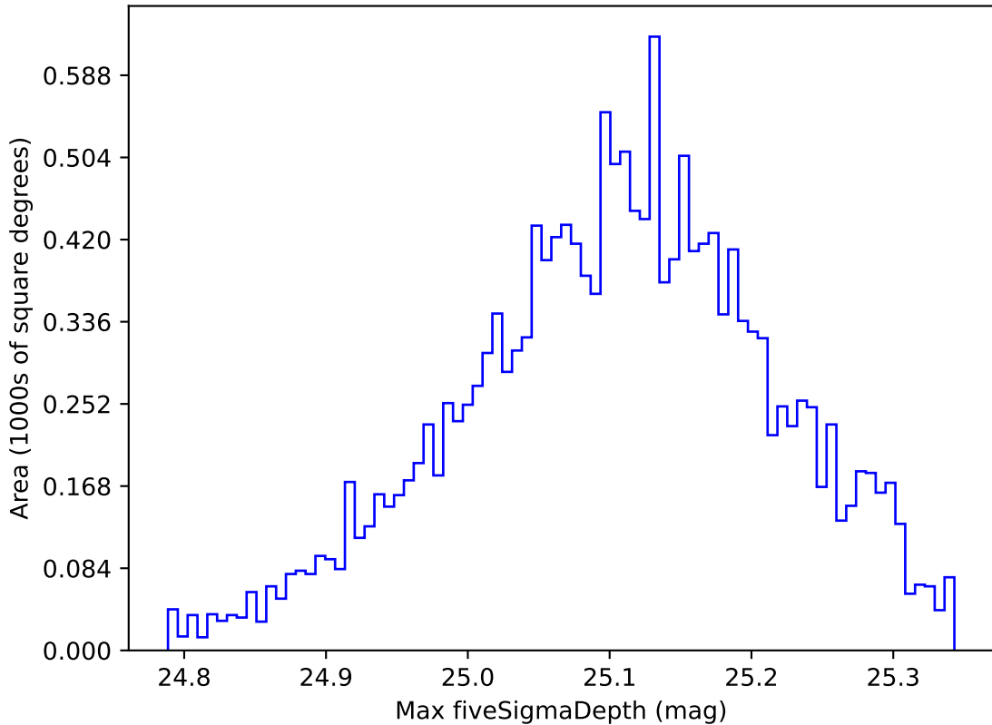
too_elab_r32_d2_giz_v3.4_10yrs WFD all bands: Max fiveSigmaDepth
