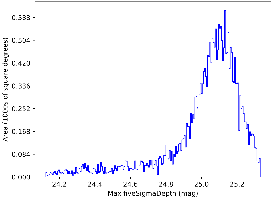
too_elab_r32_d2_giz_v3.4_10yrs All sky g band: Max fiveSigmaDepth
