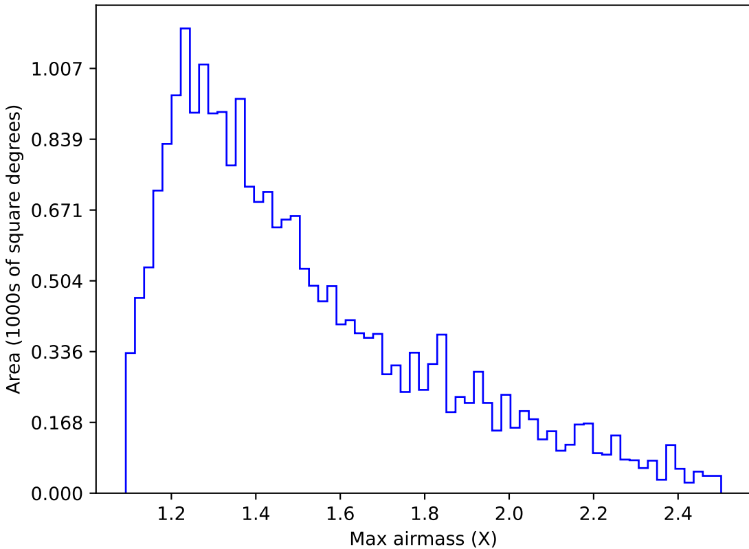
too_elab_r32_d2_giz_v3.4_10yrs Yr 1 u band: Max airmass
