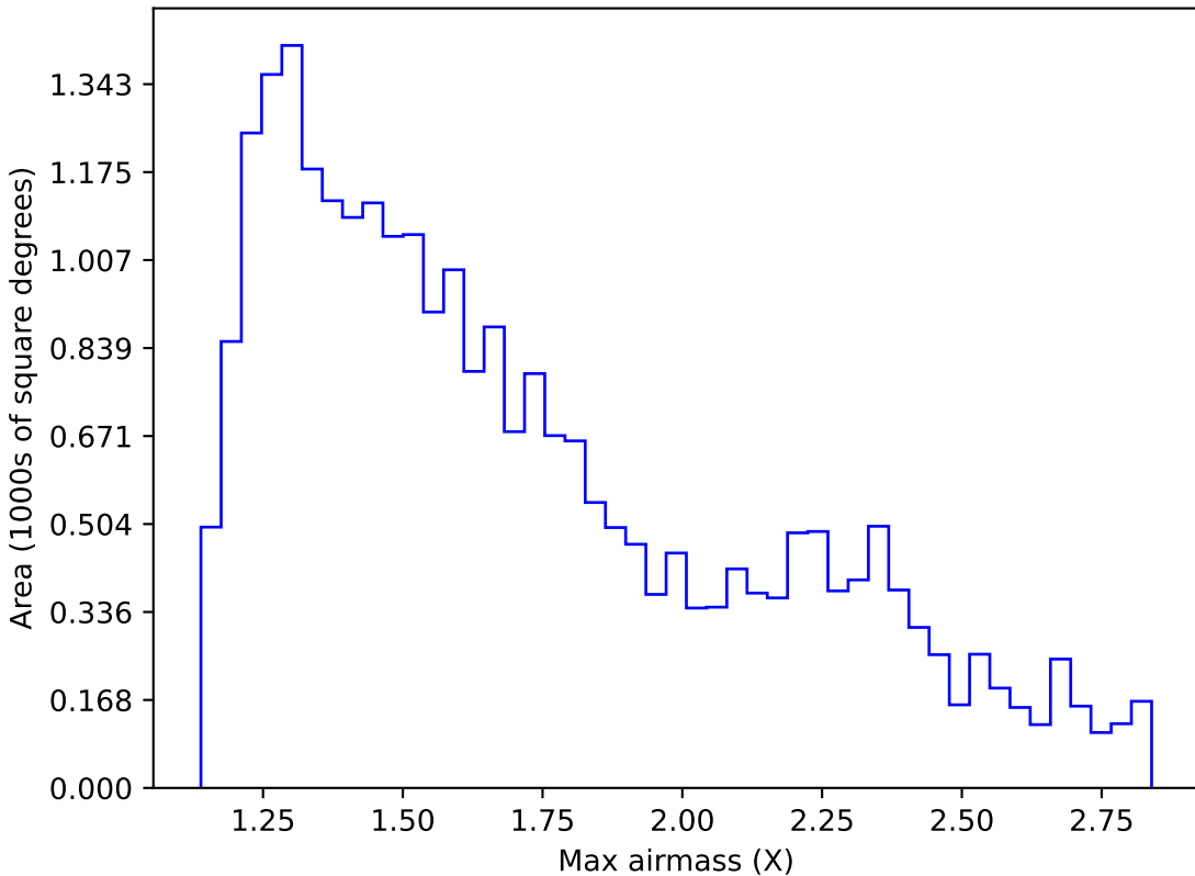
too_elab_r32_d2_giz_v3.4_10yrs Yr 1 i band: Max airmass
