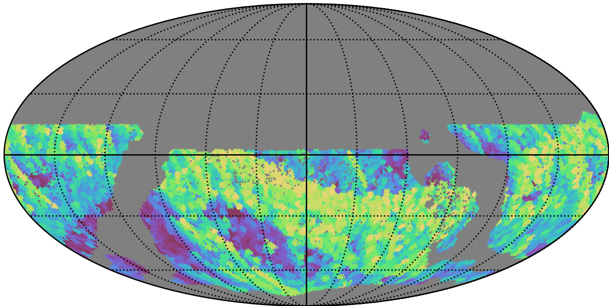
too_elab_r32_d2_giz_v3.4_10yrs WFD z band: Max airmass
